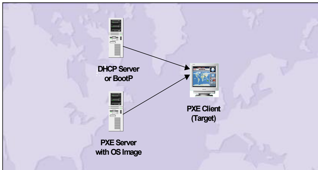
Figure 1. Typical PXE setup for Red Hat 6.2 or later Linux
