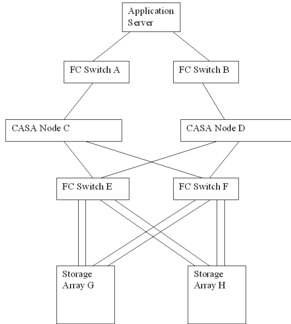
Figure 58: Single CASA Configuration
