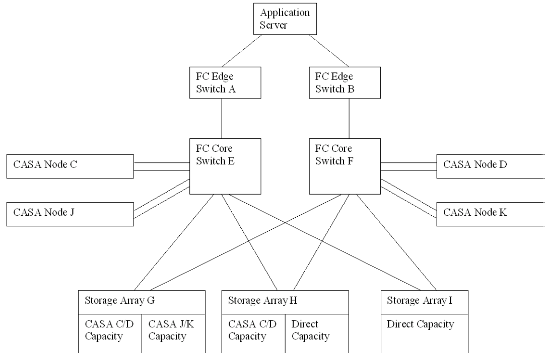
Figure 60: Multiples CASA Supporting Mix of Arrays
