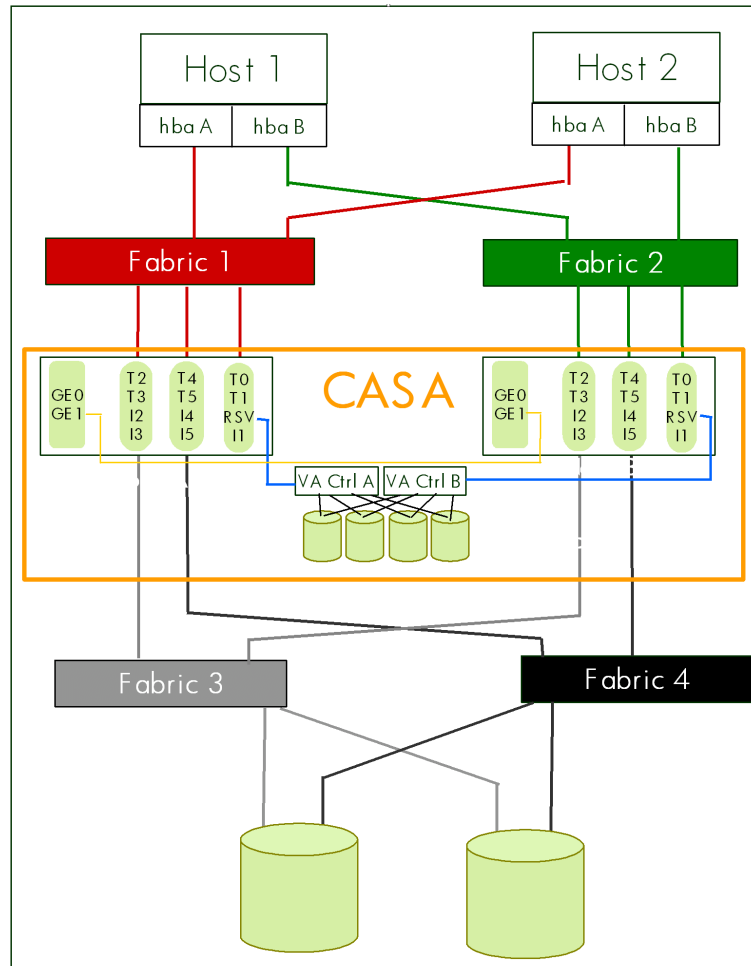
Figure 56: CASA Internal Architecture
