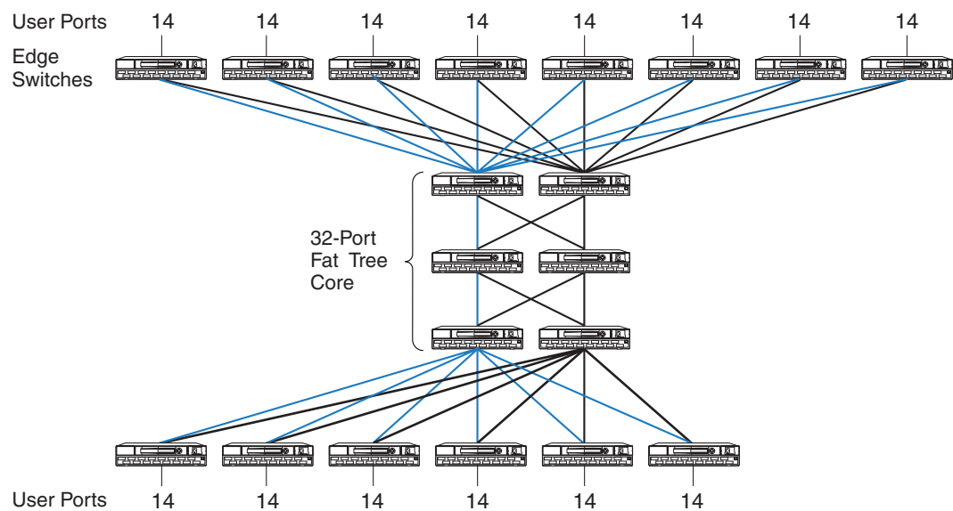
Figure 62: Example of Core Switch Plus Edge Switch Configuration
