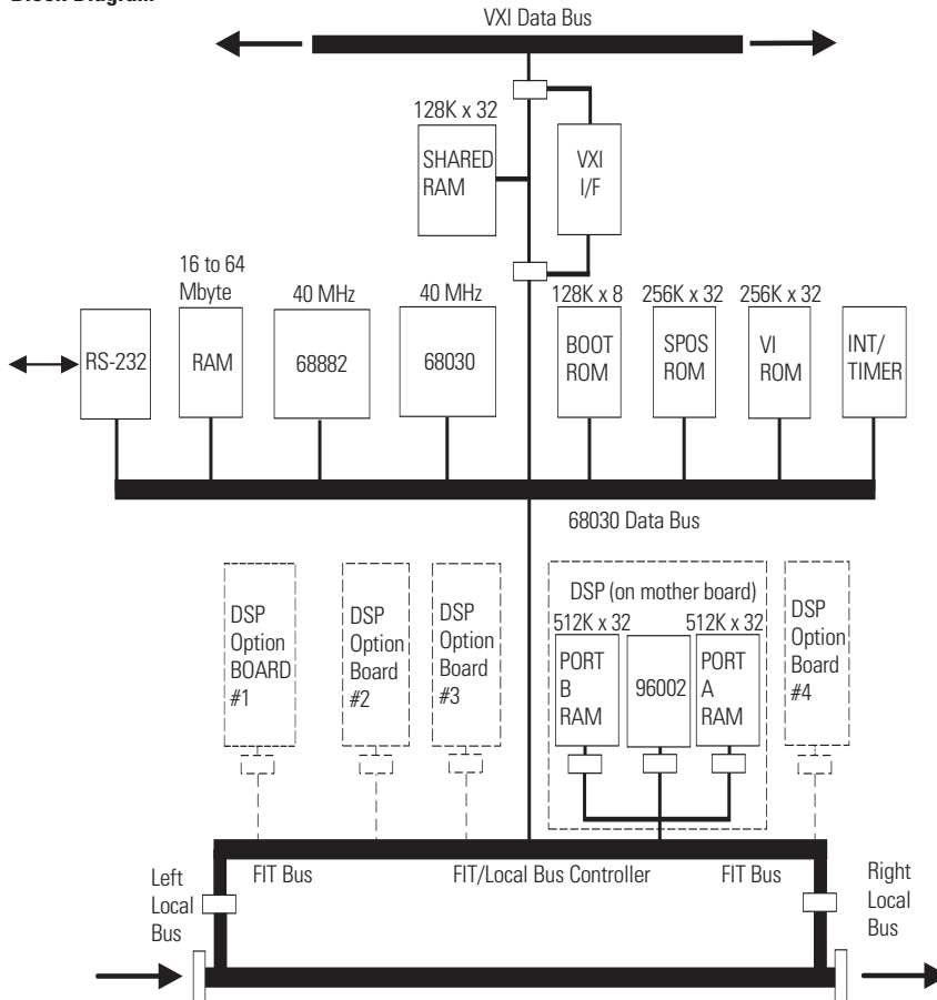
Agilent E1485C Functional Block Diagram
