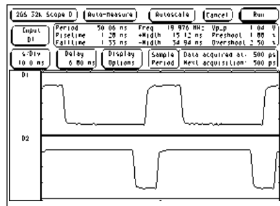
Figure 16. Oscilloscope
