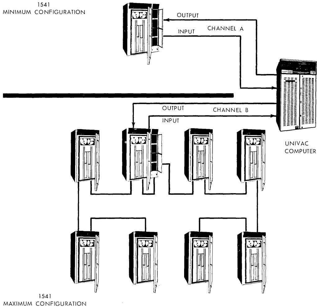
Figure 3b. UNIVAC 1541 Magnetic Tape Units and Computer Configuration
