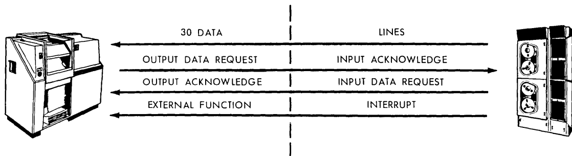
Figure 16. Magnetic Tape - Printer Interface
