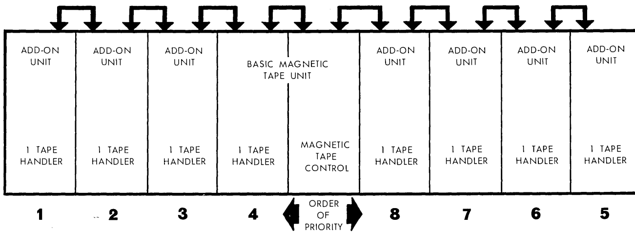
Figure 8. Type 1541 Magnetic Tape System (Maximum Configuration)
