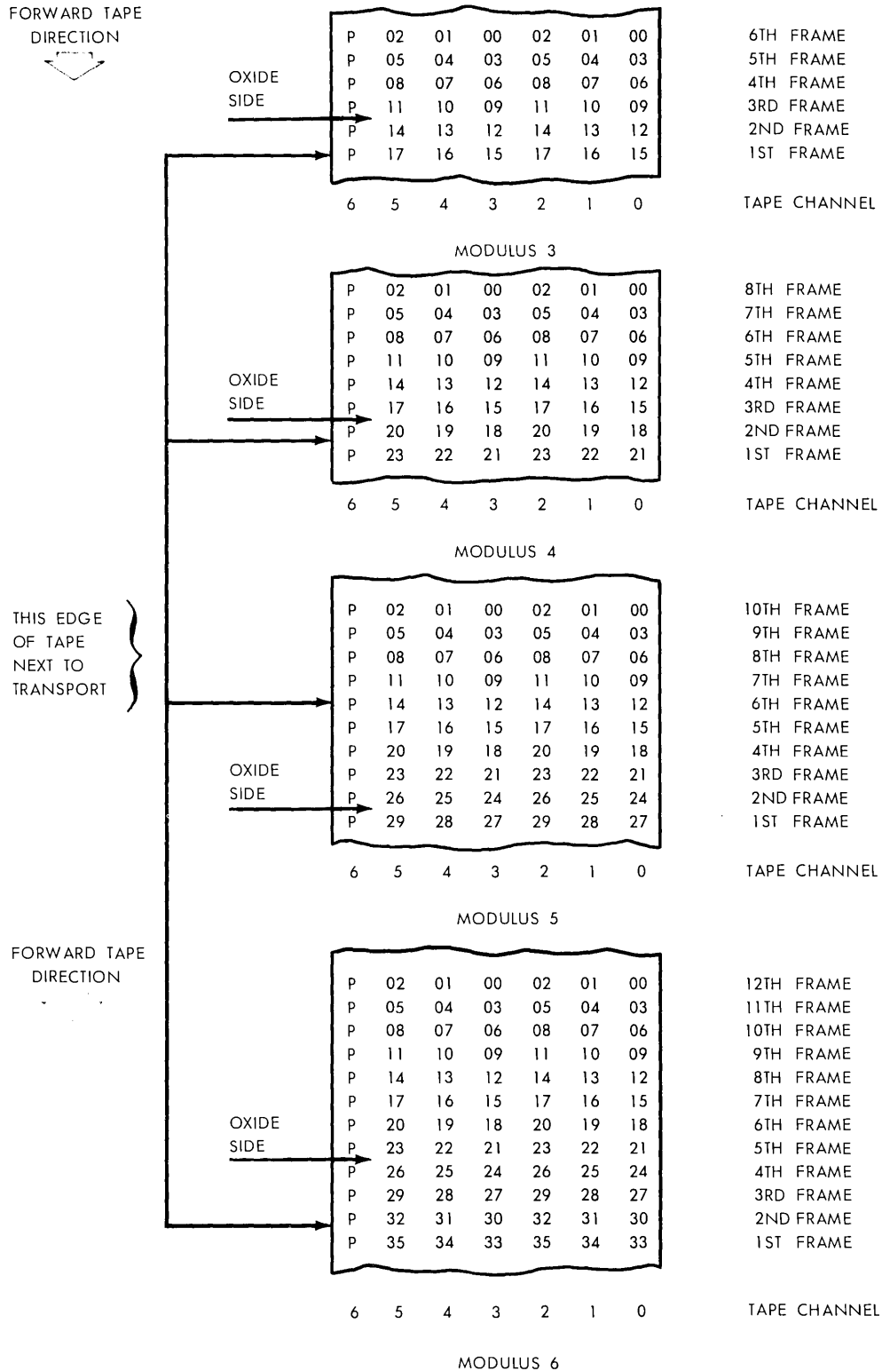
Figure 13. Octal Tape Format
