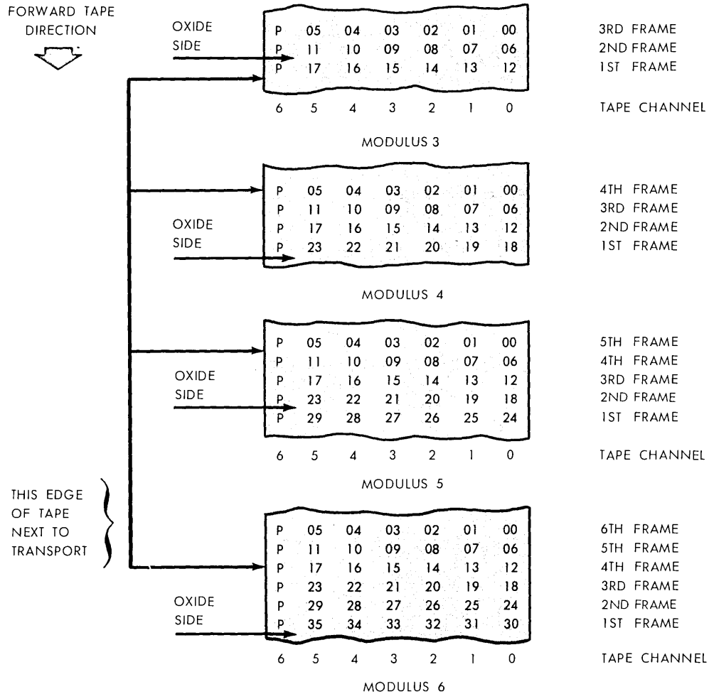
Figure 12. Bi-octal Tape Format
