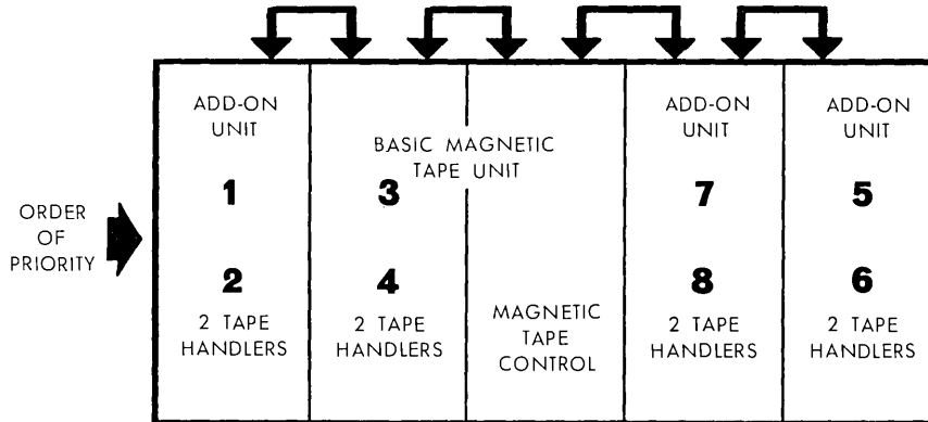
Figure 7. Type 1540 Magnetic Tape System (Maximum Configuration)
