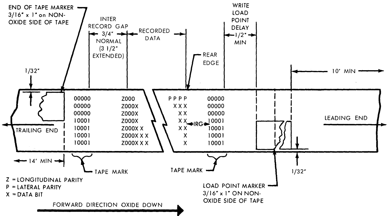
Figure 9. Tape Format
