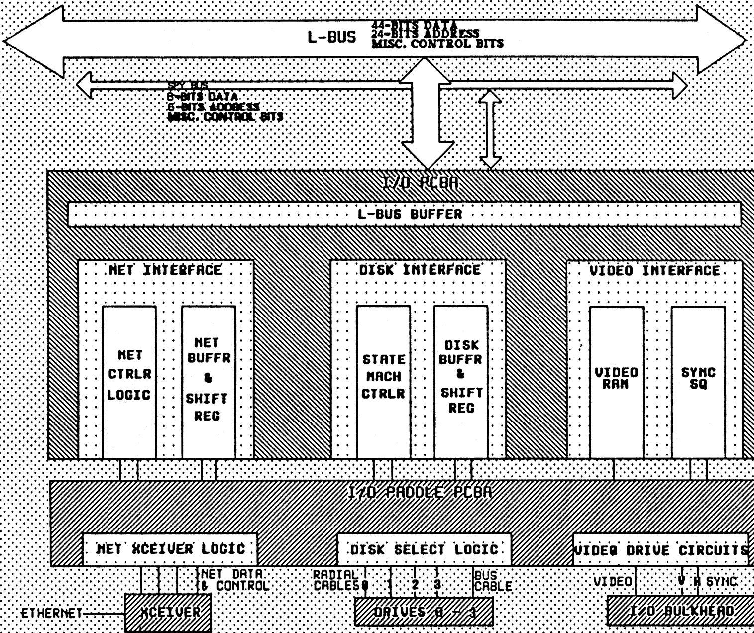
LISP I/O BLOCK DIAGRAM
