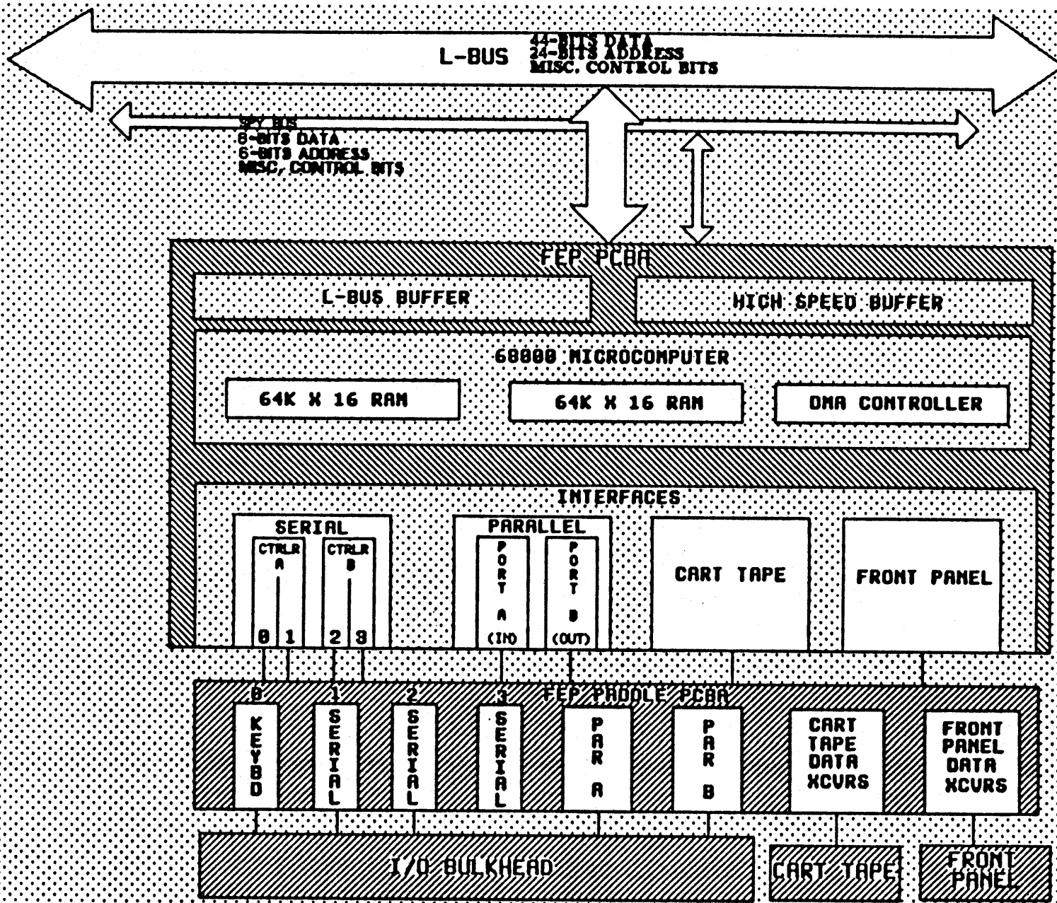
LISP FRONT END PROCESSOR BLOCK
