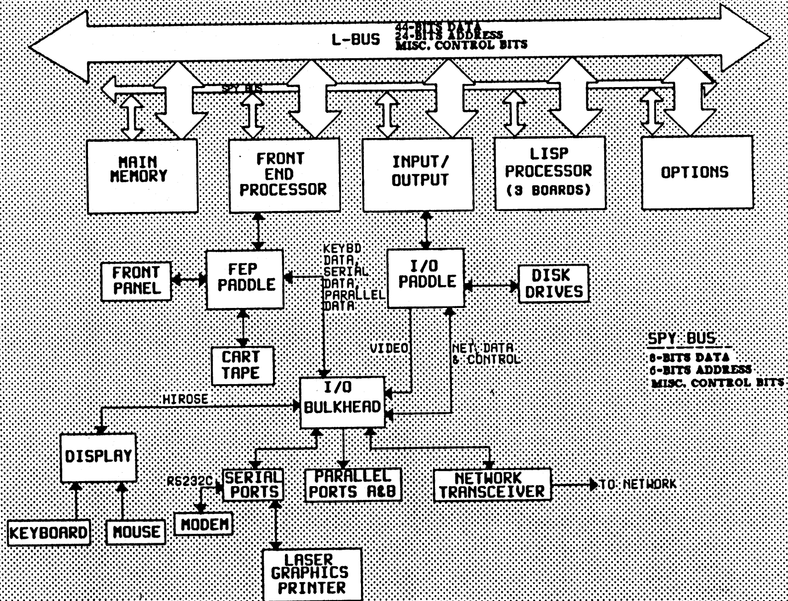
LISP SYSTEM BLOCK DIAGRAM
