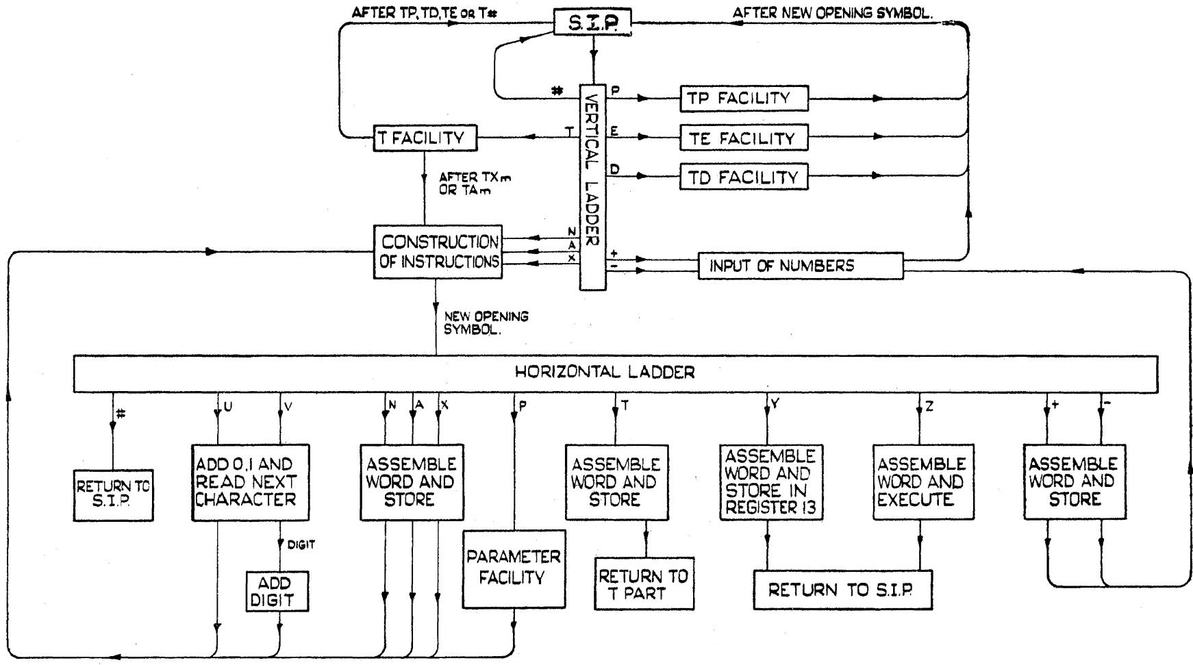
THE COMPLETE NIP BLOCK DIAGRAM IS AS FOLLOWS:-
