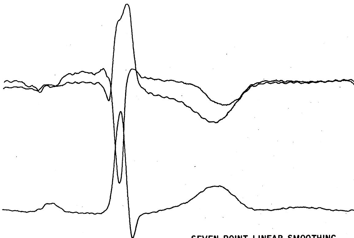
SEVEN POINT LINEAR SMOOTHING
