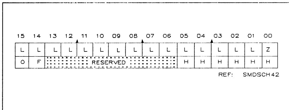
Figure 4-2: Descriptor Format
