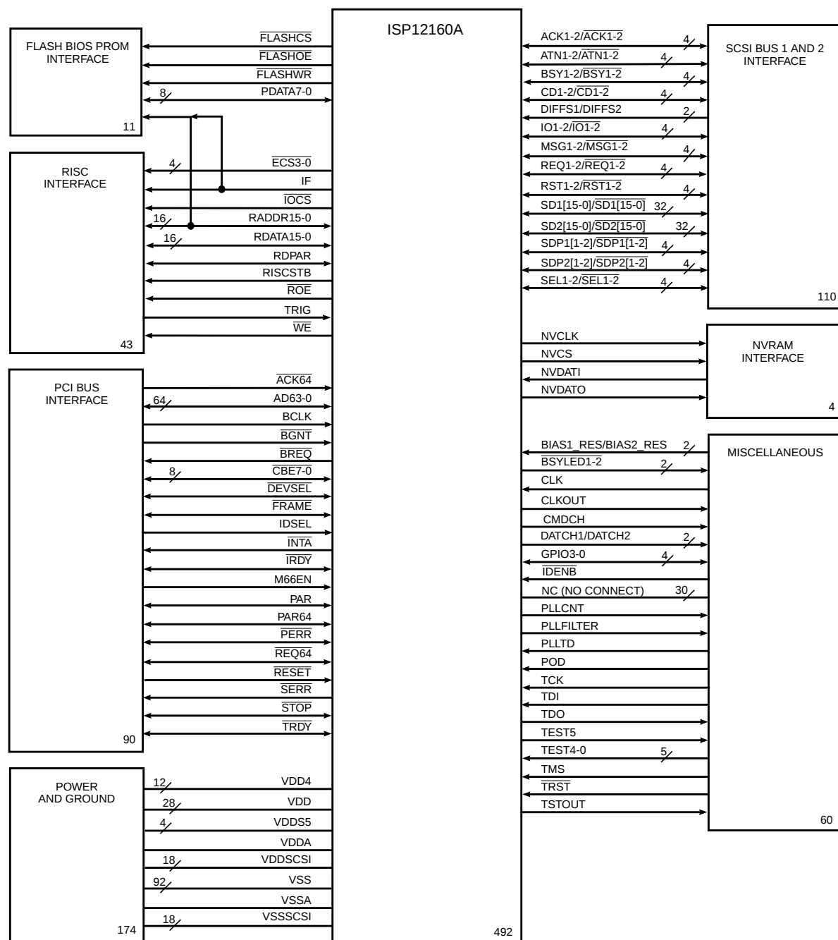
Figure 3. ISP12160A Functional Signal Grouping
