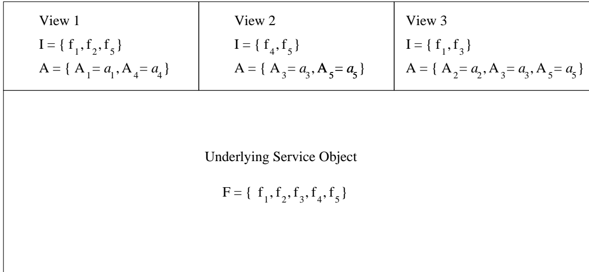
Figure 4-1: A service and its views. F is the total set of functions supported by the service. For each view, A is the set of attributes, and interface I is the subset of F that the view makes available.
