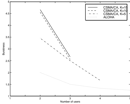
Figure 18: Burstiness versus N for CSMA/CA ( K = 15, 10, and 5 ) and ALOHA.
