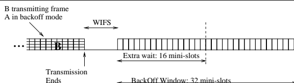
Figure 4: Illustration of WaveLAN CSMA/CA with two stations.
