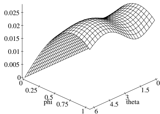
Figure 5-25: Total perspective error in the centroid. The error is expressed in pixels.
