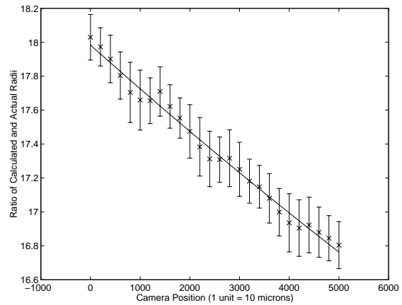
Figure 5-45: Data for dark image, camera motion in the z direction with 2000 micron steps and fiducial parallel to the image plane.
