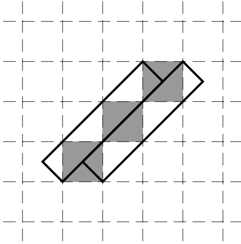
Figure 5-18: The effect of quantization errors on the centroid for a rectangular figure at an angle to the pixel lattice.
