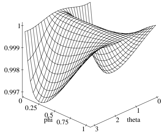
Figure 5-27: Perspective error in the semi-major axis for R_0 = 10\text{cm} . Error is expressed as the ratio of the calculated value and the actual radius.
