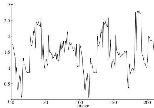
Figure 7-16: Distance in pixels between edge-based and enhanced reality positions for vertex 2.
