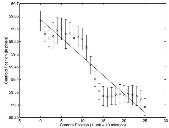
Figure 5-39: Data for bright image, camera motion in the x direction with 10 micron steps and fiducial 45^\circ to the image plane.
