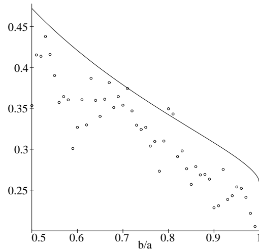
Figure 5-21: Radius error for an elliptical fiducial with a radius of 10. The error is expressed in pixels and b/a is the ratio of minor and major axis.
