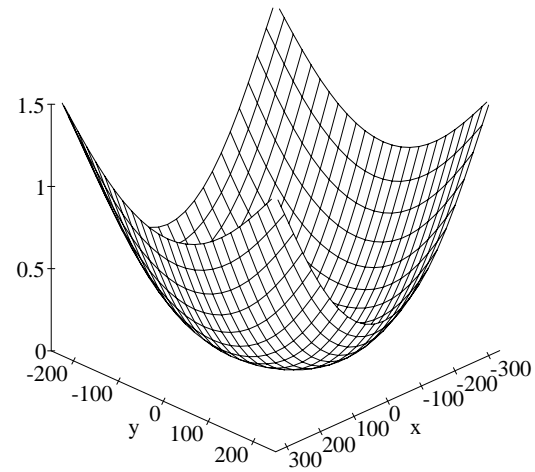
Figure A-2: Radial distortion in pixels for a 25mm lens.
