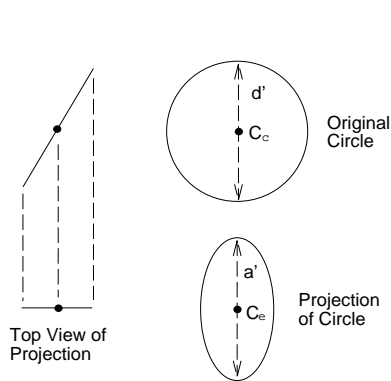
Figure 5-3: Orthographic projection of a circle.
