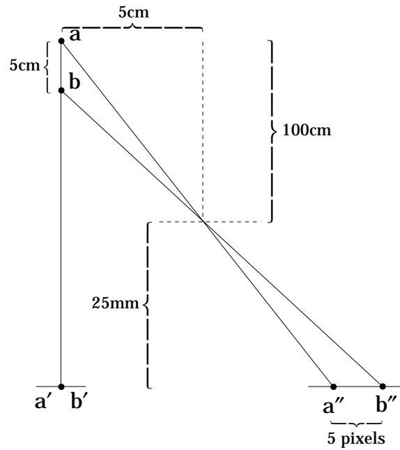
Figure 3-1: Effect of orthographic projection assumption.
