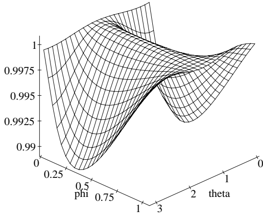
Figure 5-26: Perspective error in the semi-major axis for R_0 = 10\text{cm} . Error is expressed as the ratio of the calculated value and the actual radius.
