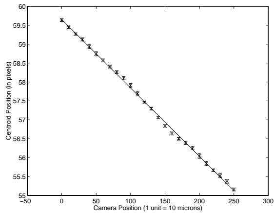
Figure 5-38: Data for bright image, camera motion in the x direction with 100 micron steps and fiducial 45^\circ to the image plane.
