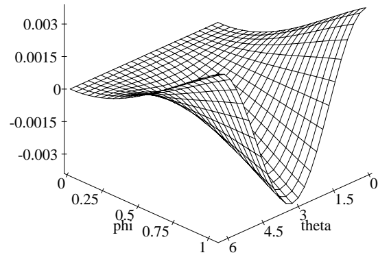
Figure 5-23: Perspective error in the centroid parallel to the major axis. The error is expressed in pixels.
