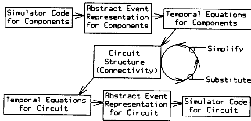
Figure 1. The FUNSTRUX system architecture. Program code for the functional models of the circuit components is converted to equations in a temporal algebra, substituted and simplified according to the circuit structure, and converted back to functional model program code for the whole circuit.
