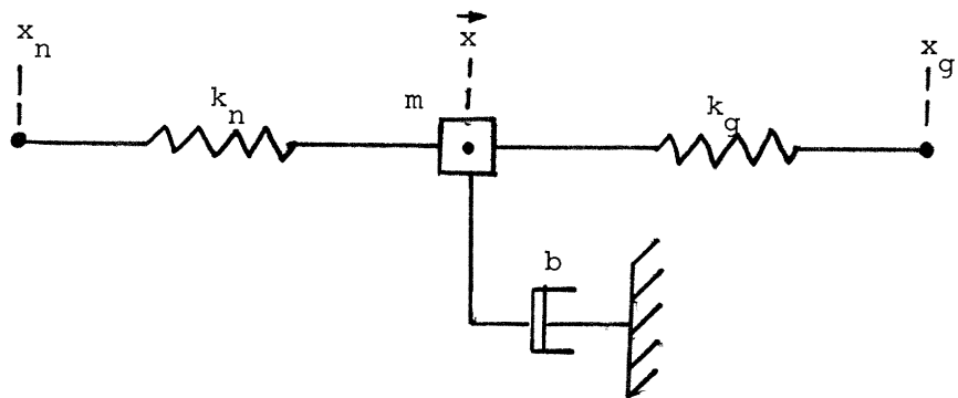
Figure 3. Simplified muscle model with equation of motion:
