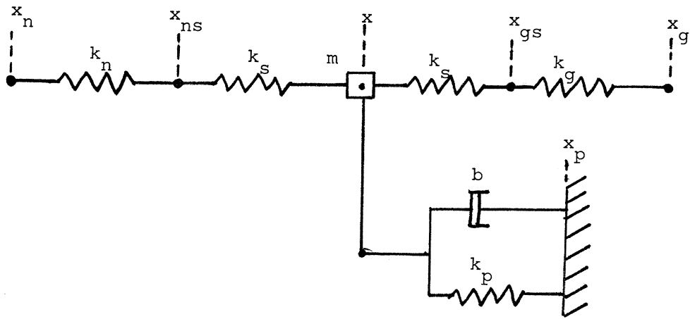
Figure 7. An expanded muscle model incorporating series elastic elements k_s and a parallel elastic element k_p .
