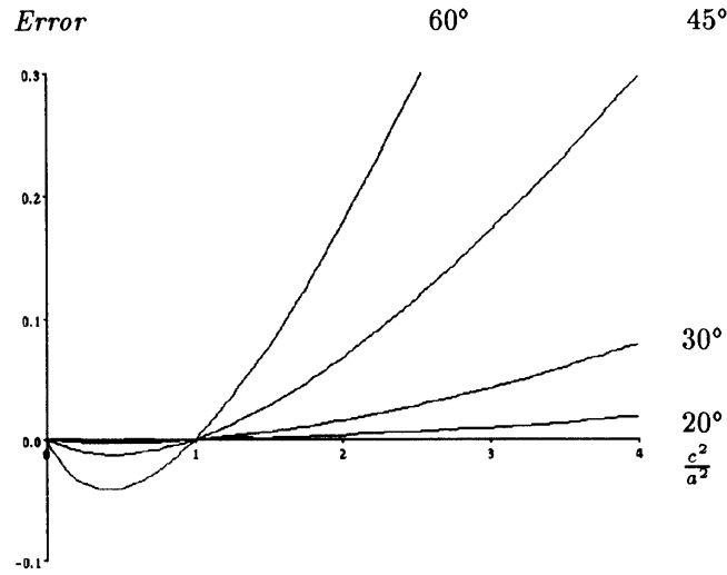
Figure 5: The error as a function of the aspect ratio, \frac{c^2}{a^2} , of the ellipsoid for \theta = 20^\circ, 30^\circ, 45^\circ , and 60^\circ . (The parameters correspond the curves at increasing magnitude.)
