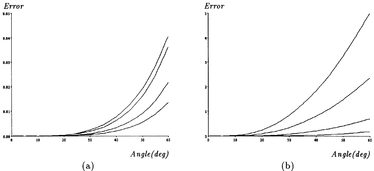
Figure 3: The errors of the curvature method as a function of \theta , the angle of rotation. (a) \frac{c^2}{a^2} = \frac{1}{16}, \frac{1}{9}, \frac{1}{4} and \frac{1}{2} . (b) \frac{c^2}{a^2} = 2, 4, 9 and 16 . (The parameters correspond the curves at increasing heights.)
