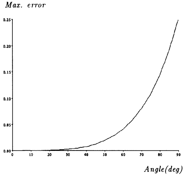
Figure 4: The maximal value of the error for canonical ellipsoids with c \leq a as a function of \theta , the angle of rotation.
