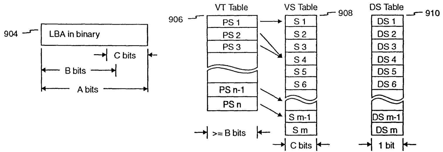
FIG. 9 LBA to PBA Mapping Architecture
