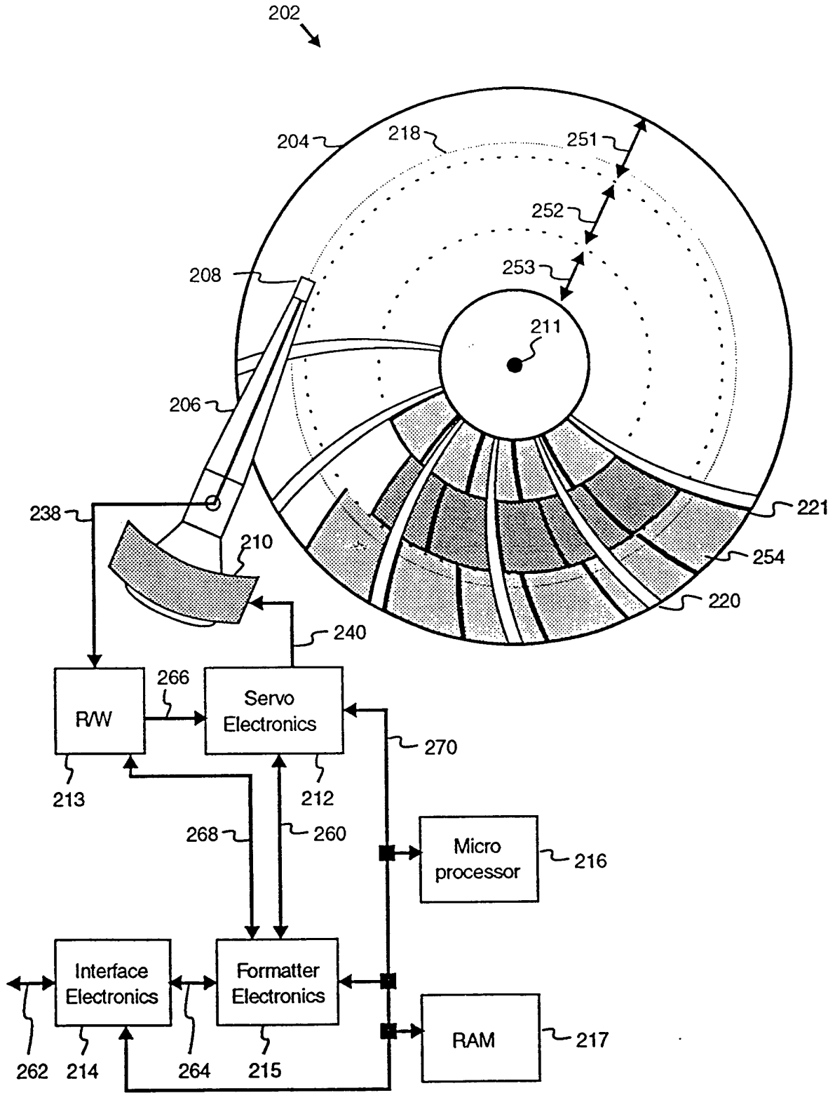
Disk Drive
