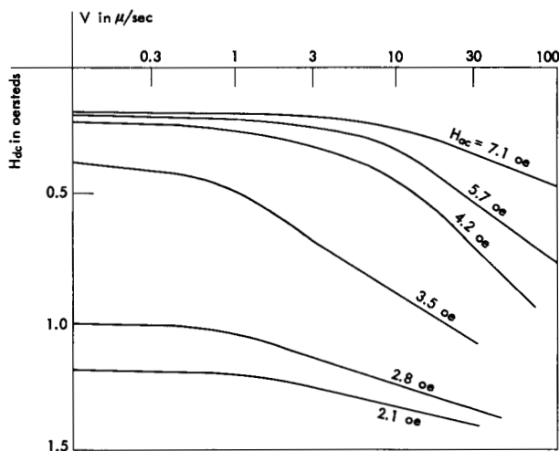
Figure 1 Velocity of domain walls in a permalloy film as a function of a dc field in the easy direction, with a 50 cps sinusoidal field in the hard direction. Values given for H_{ac} are peak values.
