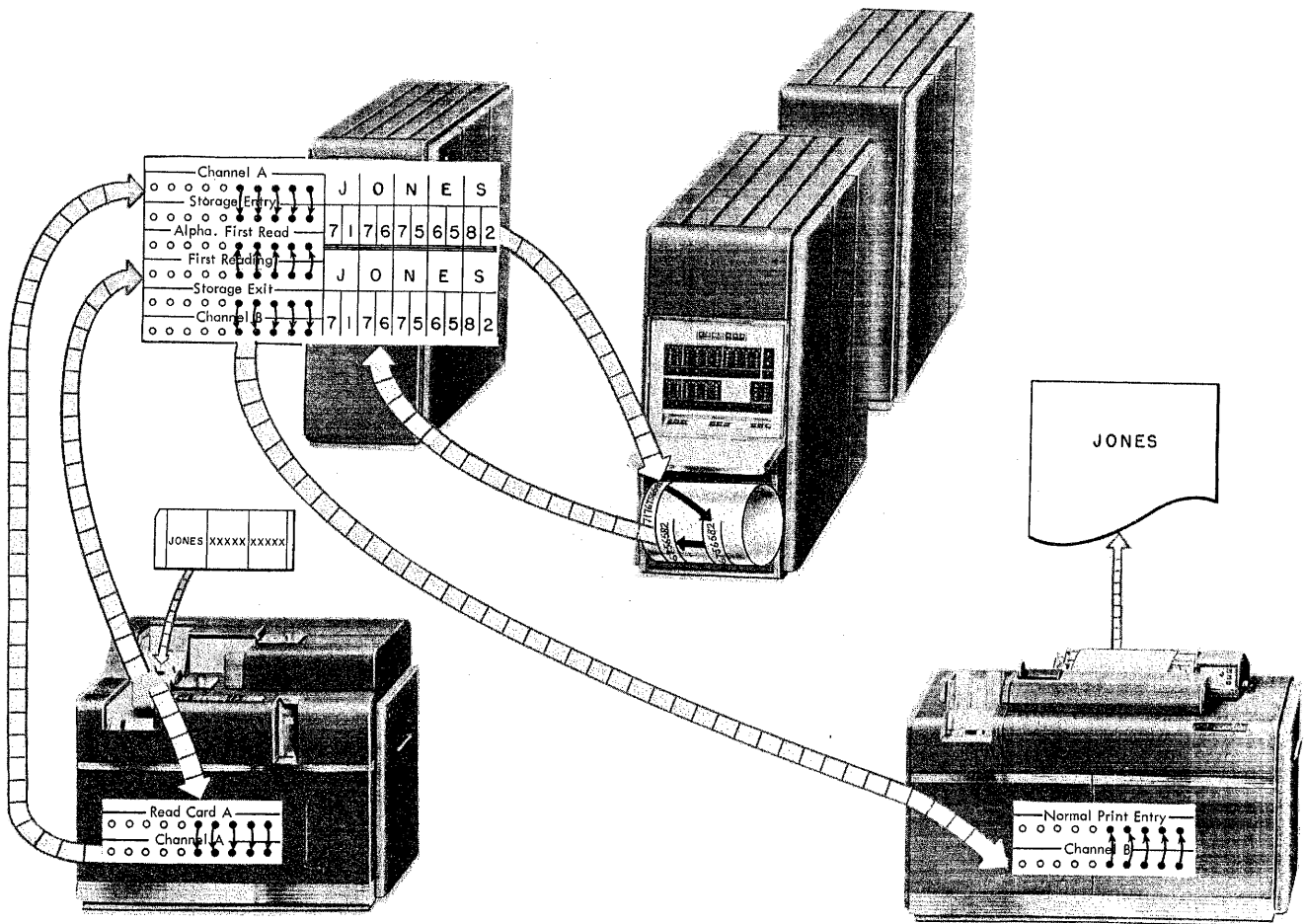
Figure 44. Data Flow Sample Application
