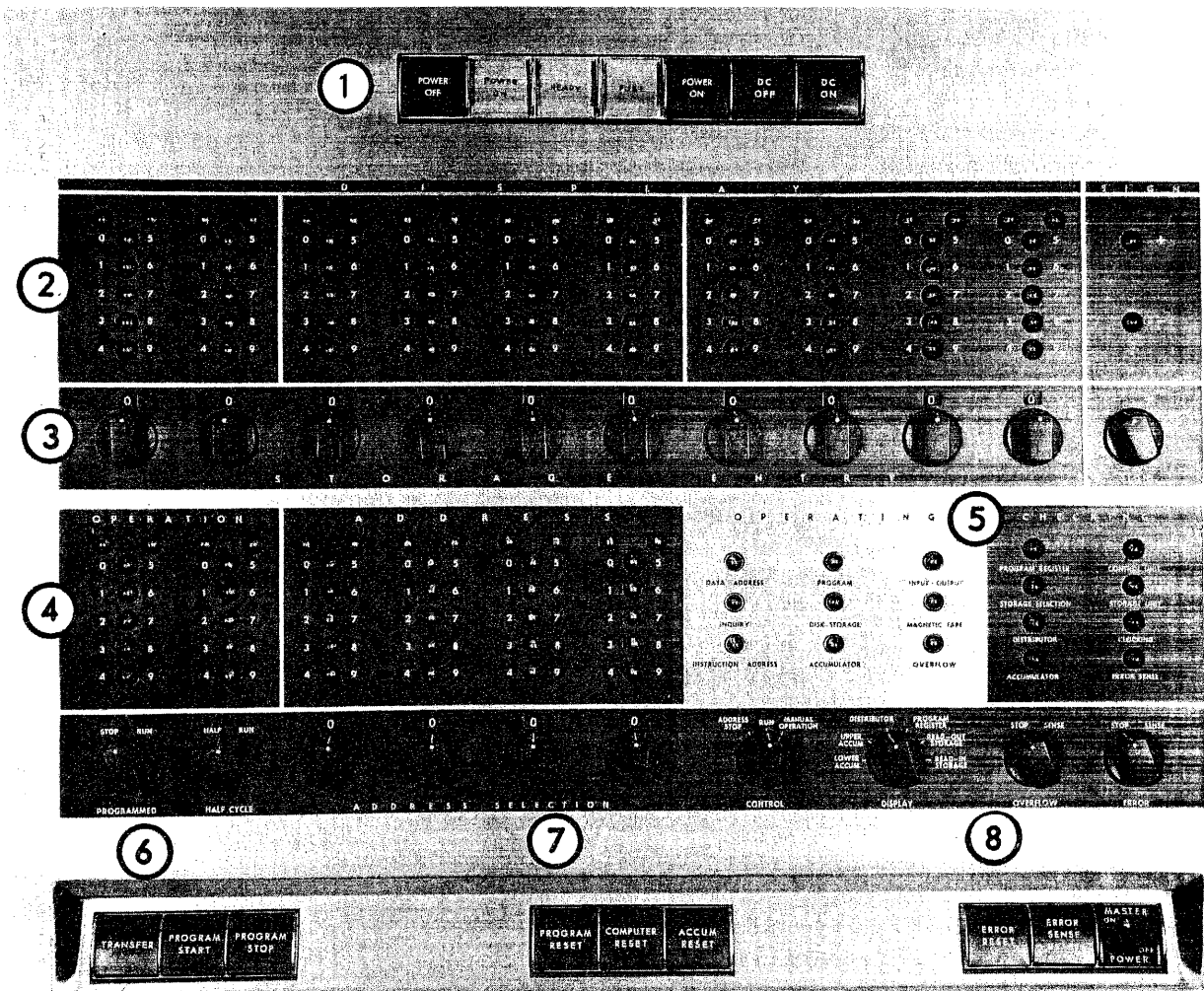
Figure 15. Control Console
