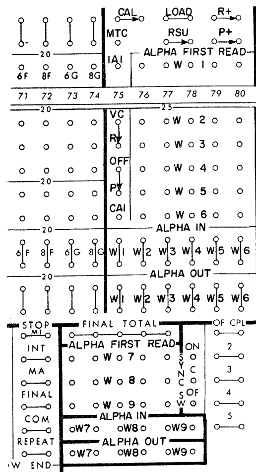
Figure 31. Alphabetic Output Control-Panel Hubs, 407
