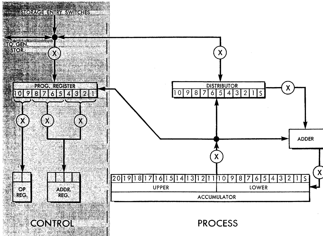
Figure 8. Process Block
