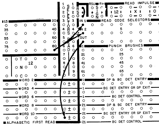
Figure 51. Read Code Selectors with RSO
