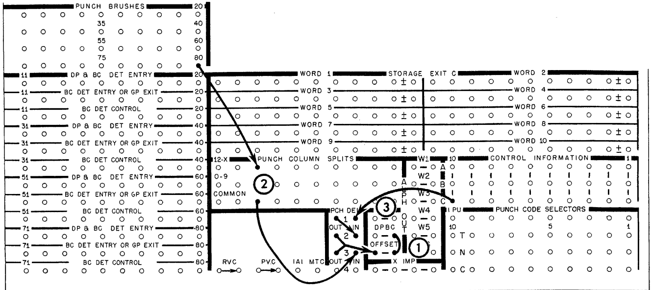
Figure 48. Offset Stacking, 533
