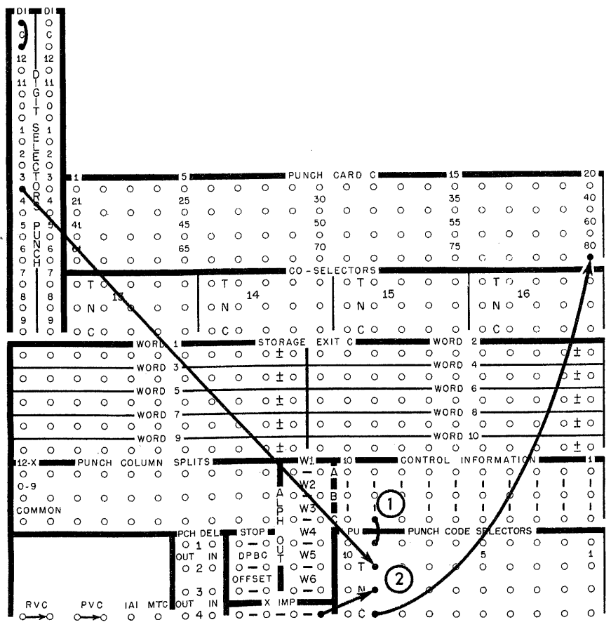
Figure 52. Punch Code Selectors
