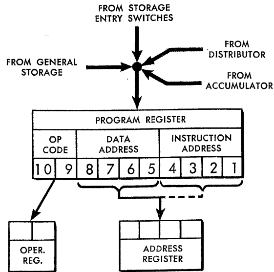
Figure 10. Program Register
