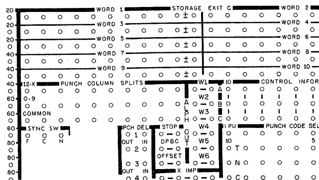
Figure 30. Alphabetic Output Control-Panel Hubs, 533-537
