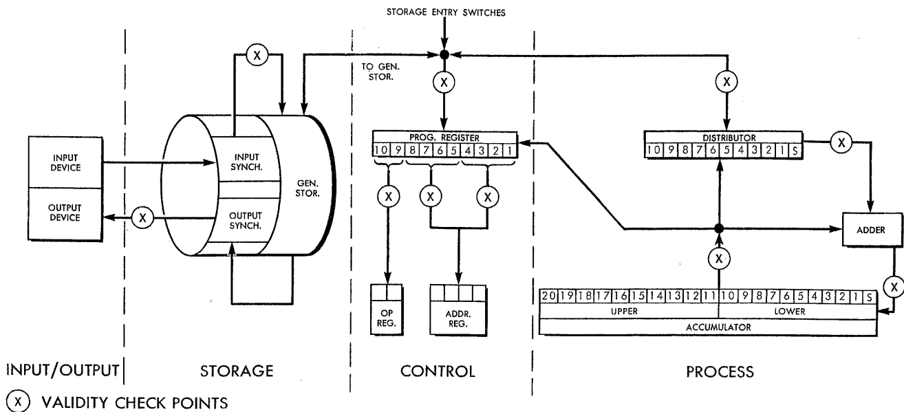
Figure 12. Flow Paths and Validity Check Points
