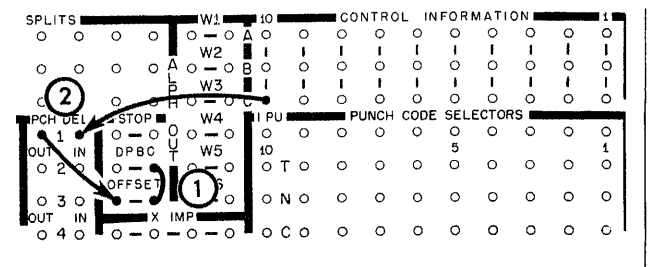
Figure 49. Offset Stacking, 537
