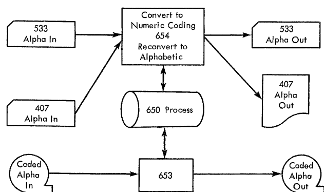
Figure 34. Alphabetic Data Flow Schematic
