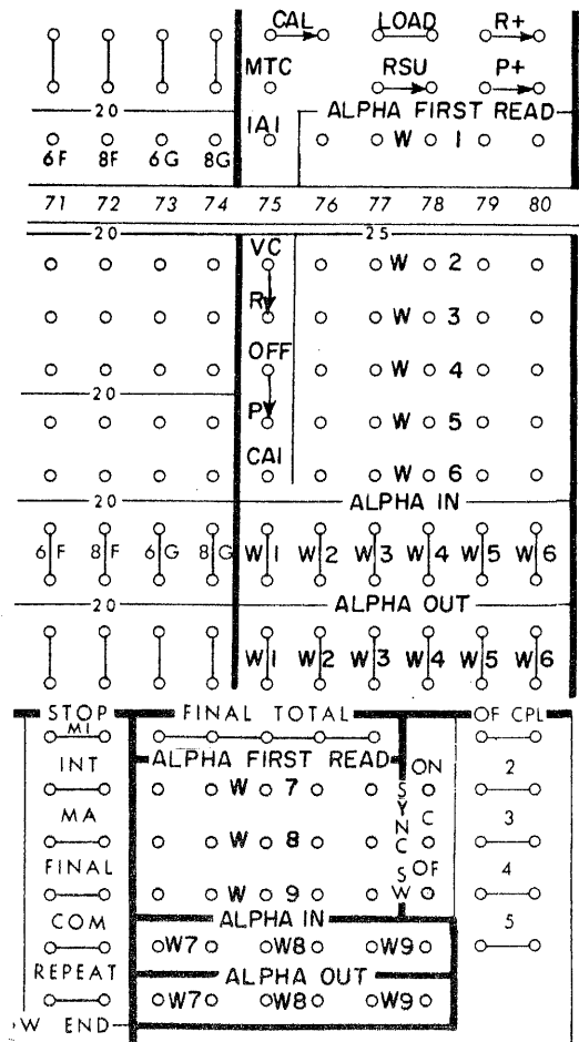
Figure 26. 407 Control-Panel Hubs—Alphabetic Input
