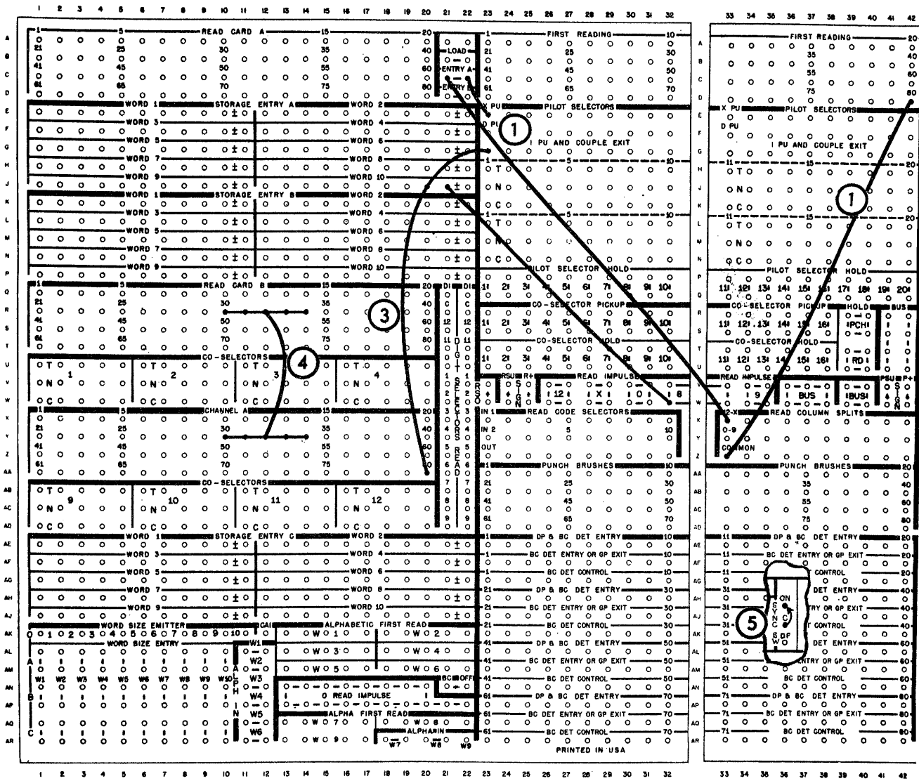
Figure 45. 533 Control Panel Wiring
