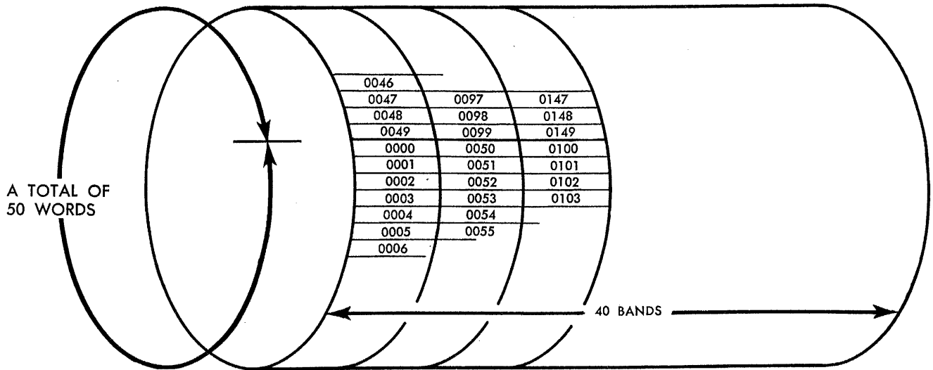
Figure 6. Magnetic Drum Storage Location Layout
