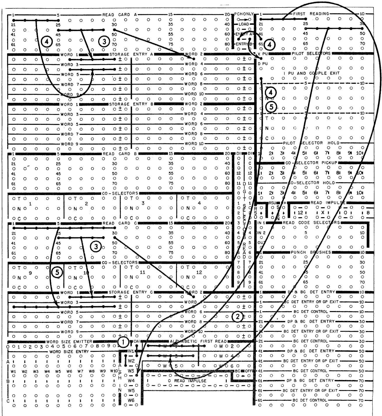
Figure 27. Alphabetic Input, 533-537
