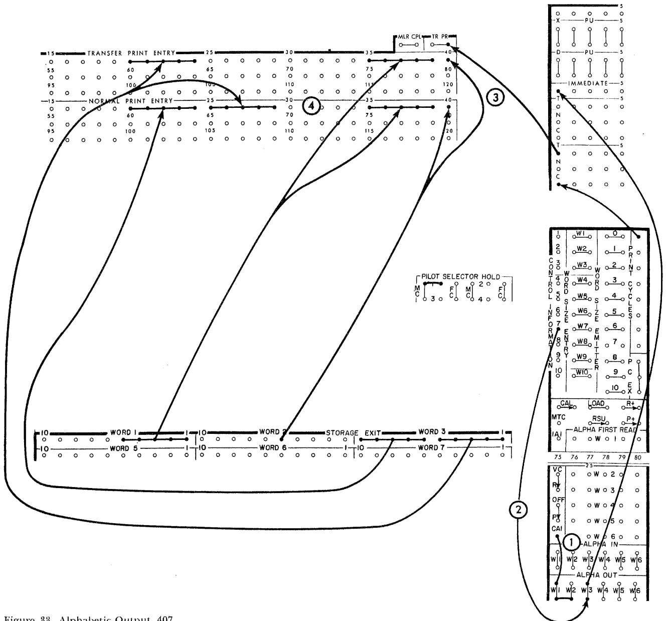
Figure 33. Alphabetic Output, 407
