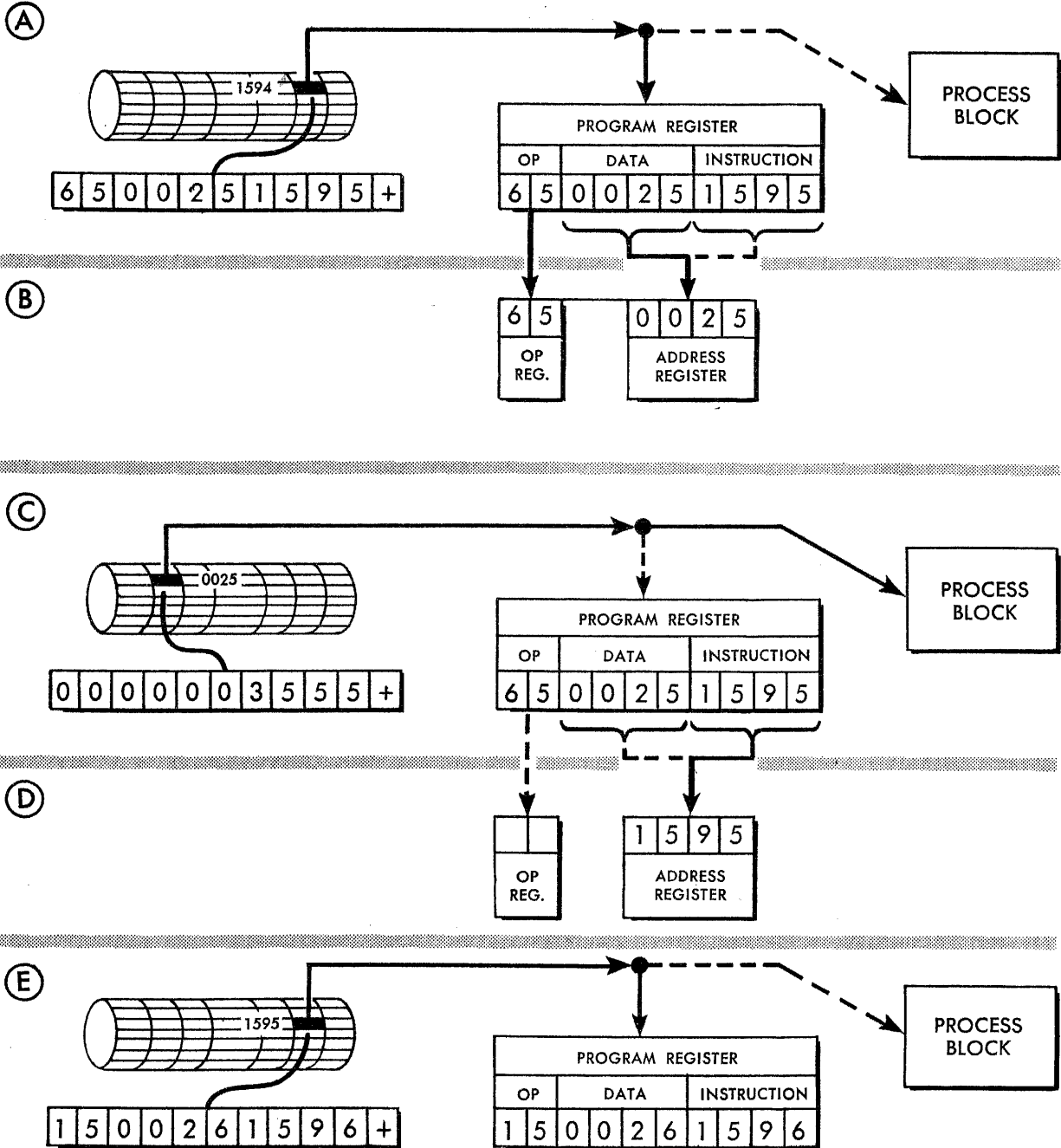
Figure 11. Instruction Execution
