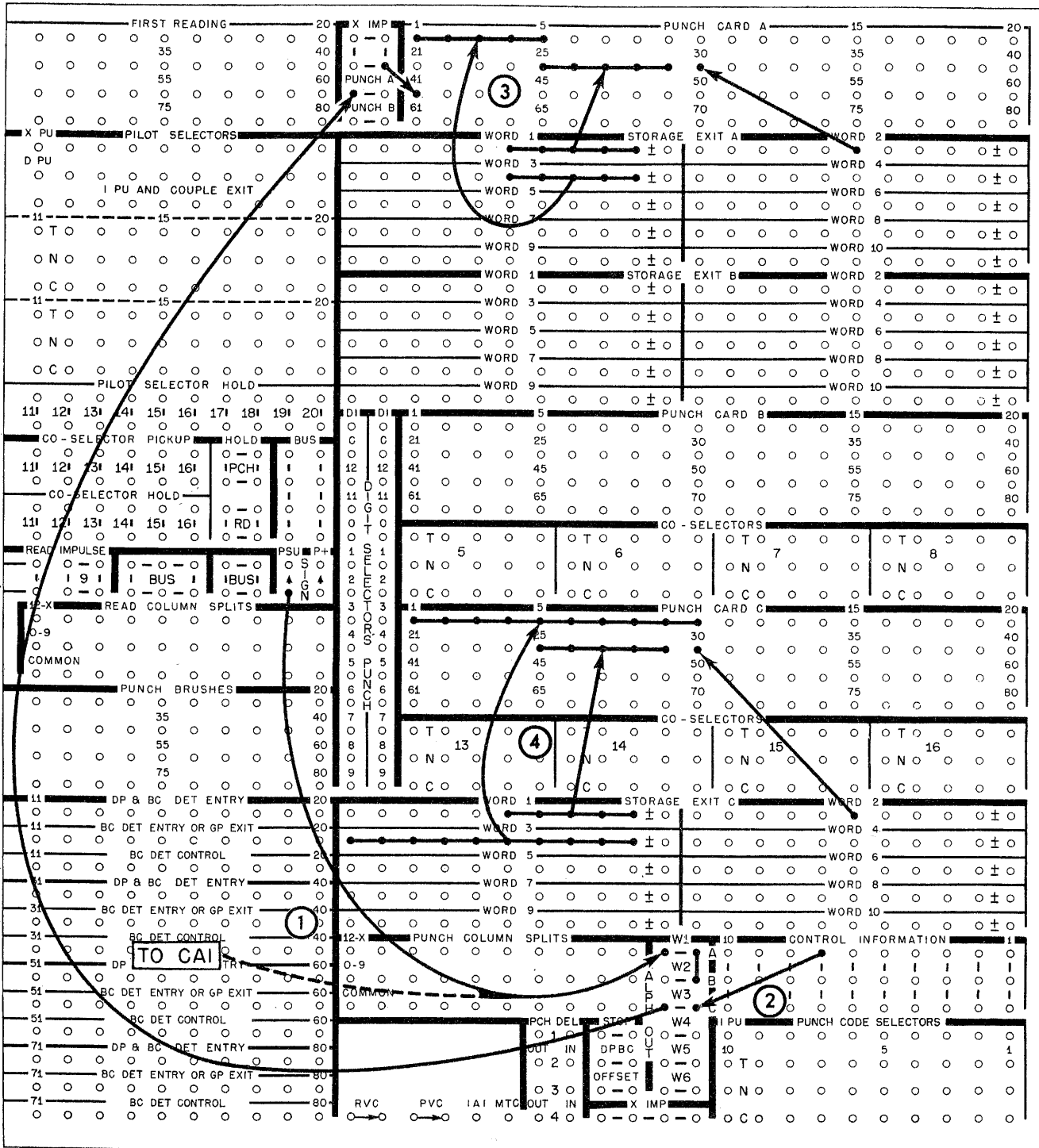
Figure 32. Alphabetic Output, 533-537
