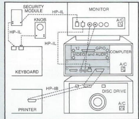
CONFIGURATION FOR 59970C OPTION #120
