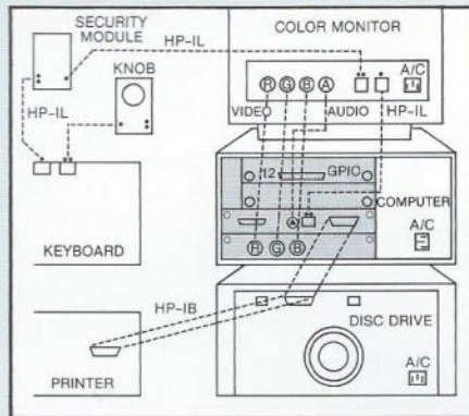
CONFIGURATION FOR 59970C OPTION #140
