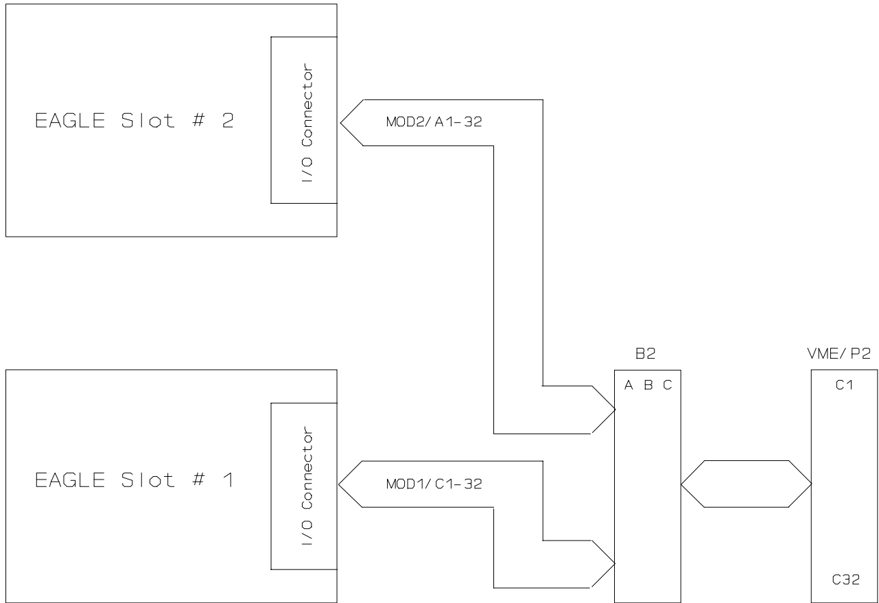
Figure 5: Block Diagram of the EAGLE I/O Connectors to the VME/P2
