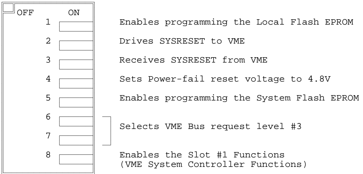
slide switch SW5
