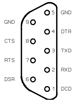
B) Micro D-Sub and D-Sub Female Connectors on the Adapter/Terminal Cable
