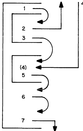
Figure 14 Program Branching in DO Loops
