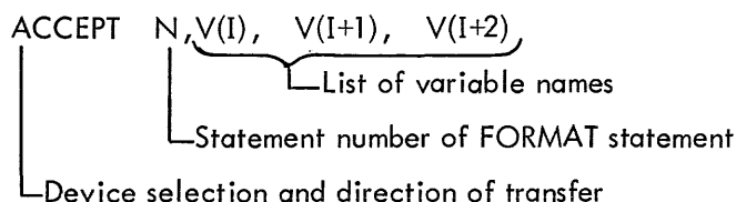
Figure 15 Input/Output Statement
