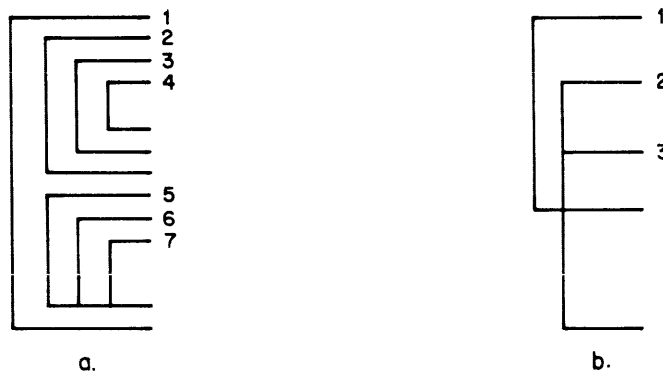
Figure 13 DO Loops
