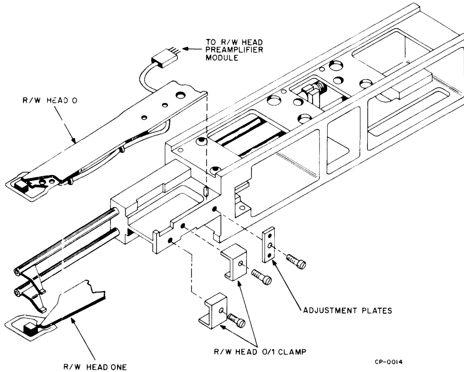
Figure 2-4 Read/Write Carriage Assembly Diagram
