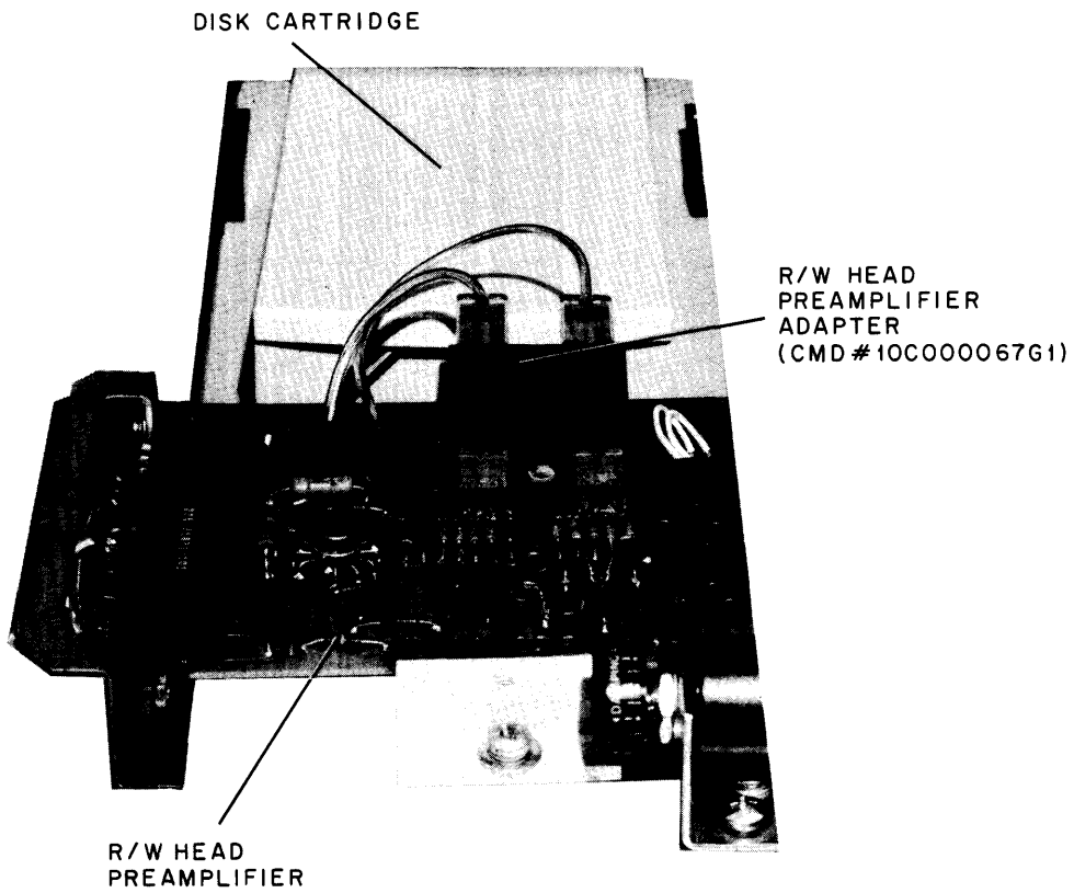
Figure 6-2 Electronic Module Assembly Diagram
