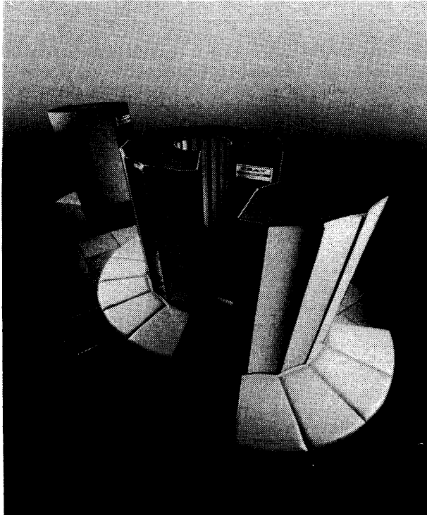
The X-MP/4 systems include 4 central processors with 32, 64, or 128 megabytes of main memory. In this photograph, the main-frame is in the center. To the left is the I/O subsystem and to the right is a Solid-State Storage Device.
