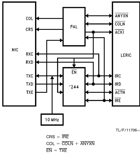
FIGURE 2. LERIC-NIC Interface
