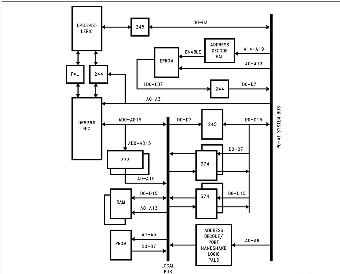
FIGURE 1. LERIC-NIC PC-AT System Interface
