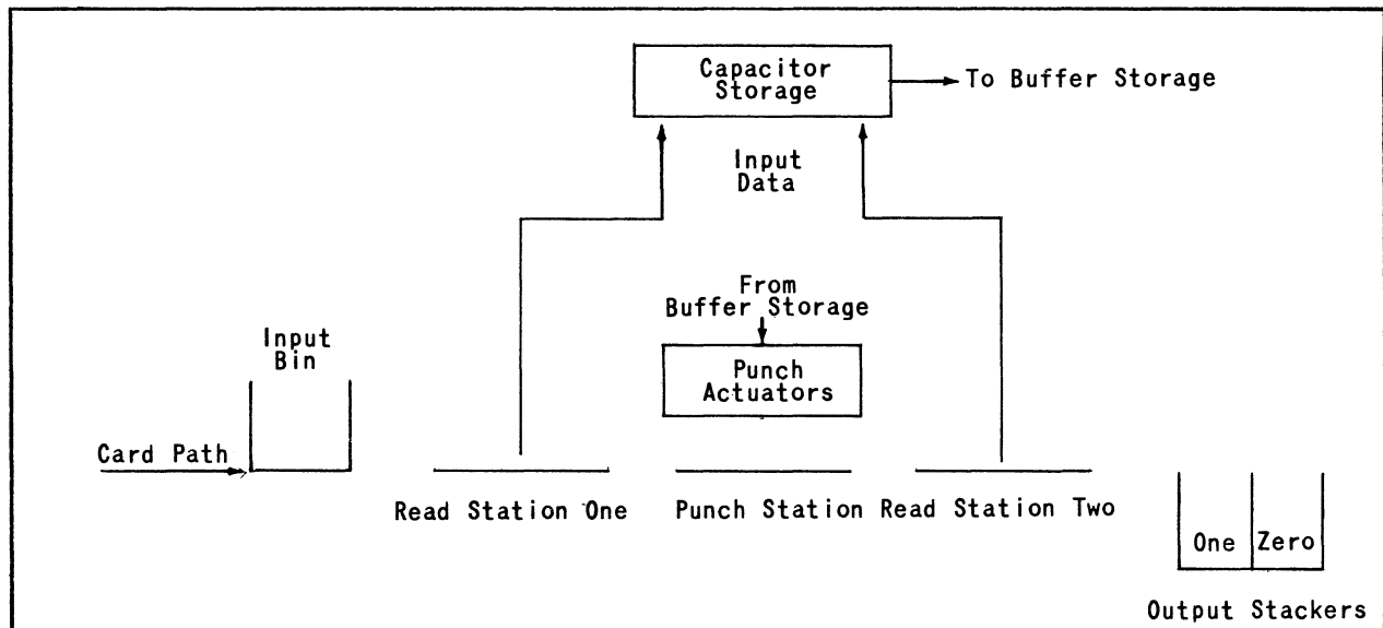
Figure 15 Read-Punch Unit
