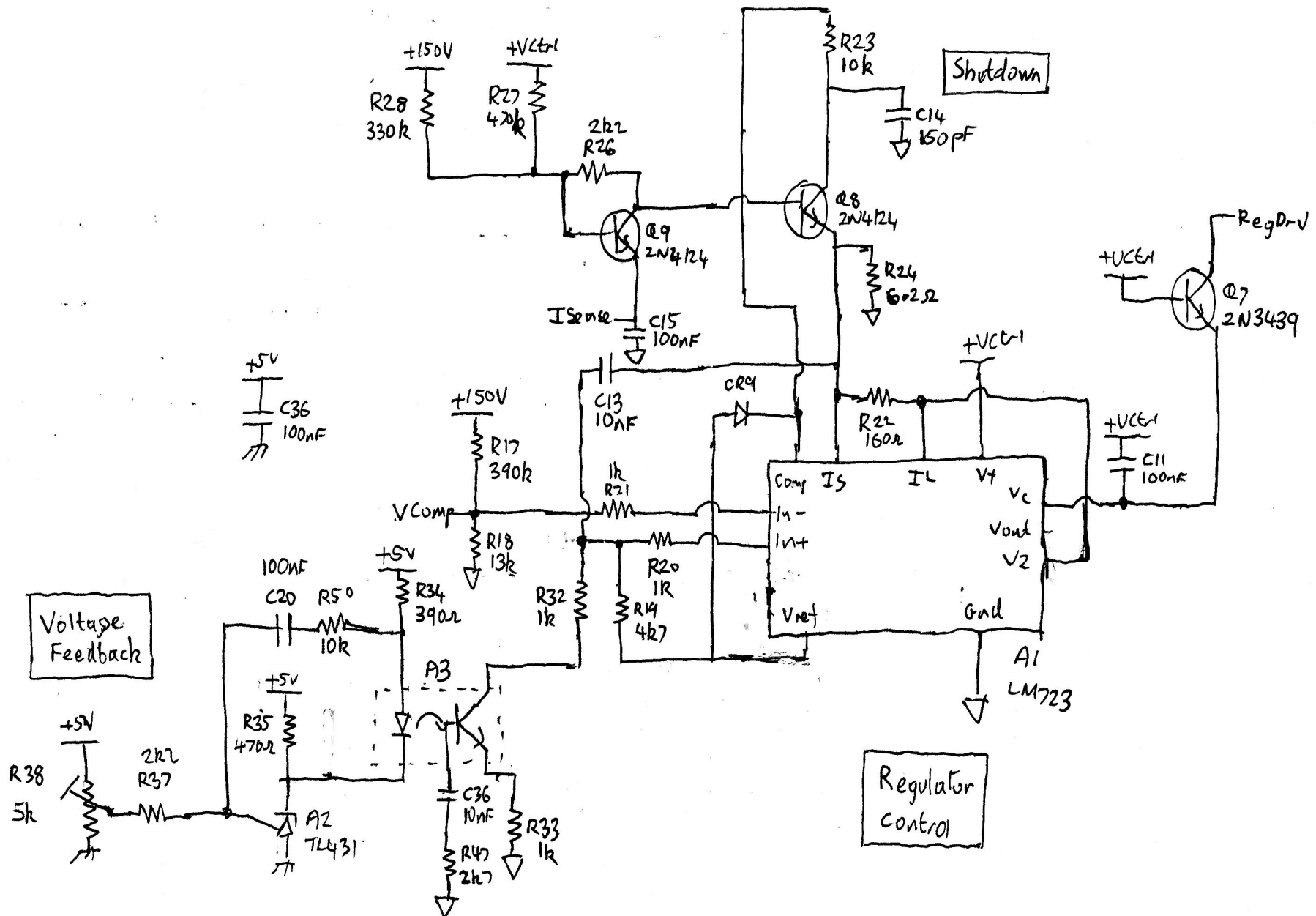
Boschert 0L130 PSU sheet (4)
